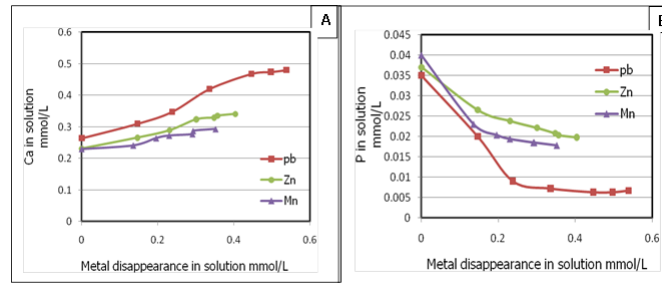
Figure 5. Calcium (A) and Phosphate (B) in equilibrium solution as a function of heavy metal disappearance
