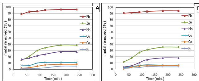
Figure 1. percentage of ions removed from wastewater by apatite mineral (A) (P1) and (B) (P2)
