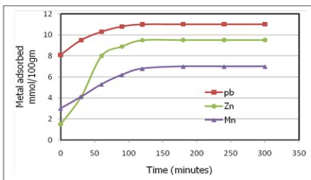
Figure 2. adsorbed amount of studied heavy metals as a function of time
