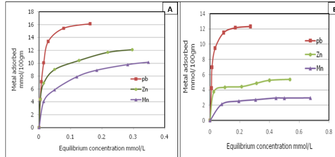
Figure 3. Adsorption isotherms of (A) mono-metal and (B) ternary-metal on apatite mineral at pH (6)
