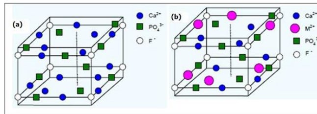
Figure 6. unit cell of apatite mineral (a) before and (b) after interaction with heavy metal ions ( M^{+2} )
