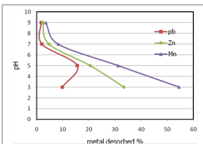
Figure 8. percentage of metal desorption as a function of pH
