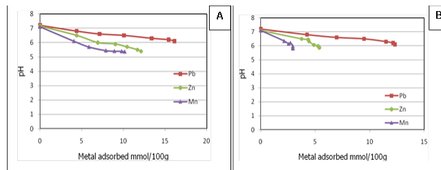
Figure 7. final pH as a function of metal adsorbed mmol/100g free control system (A) mono-metal (B) ternary –metal
