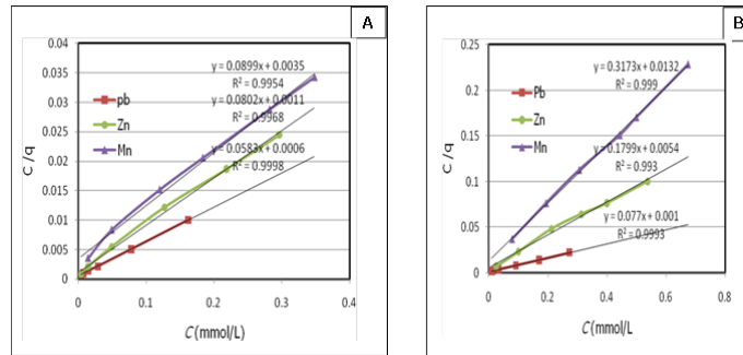
Figure 4. Langmuir adsorption isotherm of Pb^{2+} , Zn^{+2} and Mn^{+2} on apatite mineral (A) mono-metal and (B) ternary-metal
